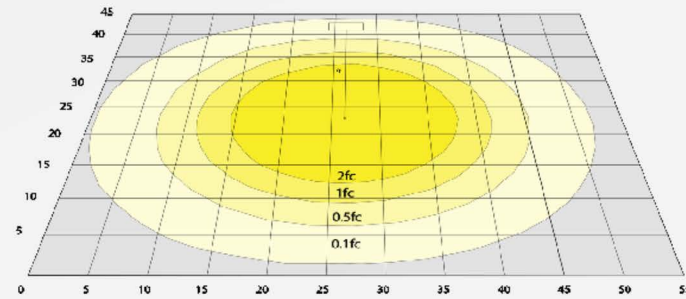
Area 45'x 55' Mounting Height: 9'
